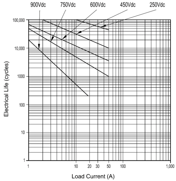
Graph-2, EVQ50 Series (Non-Polarity)
