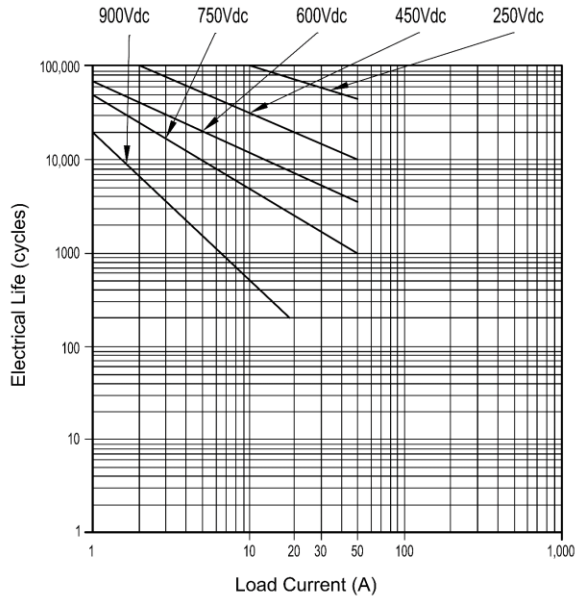
Graph-1, EVQ50 Series (Polarity)
